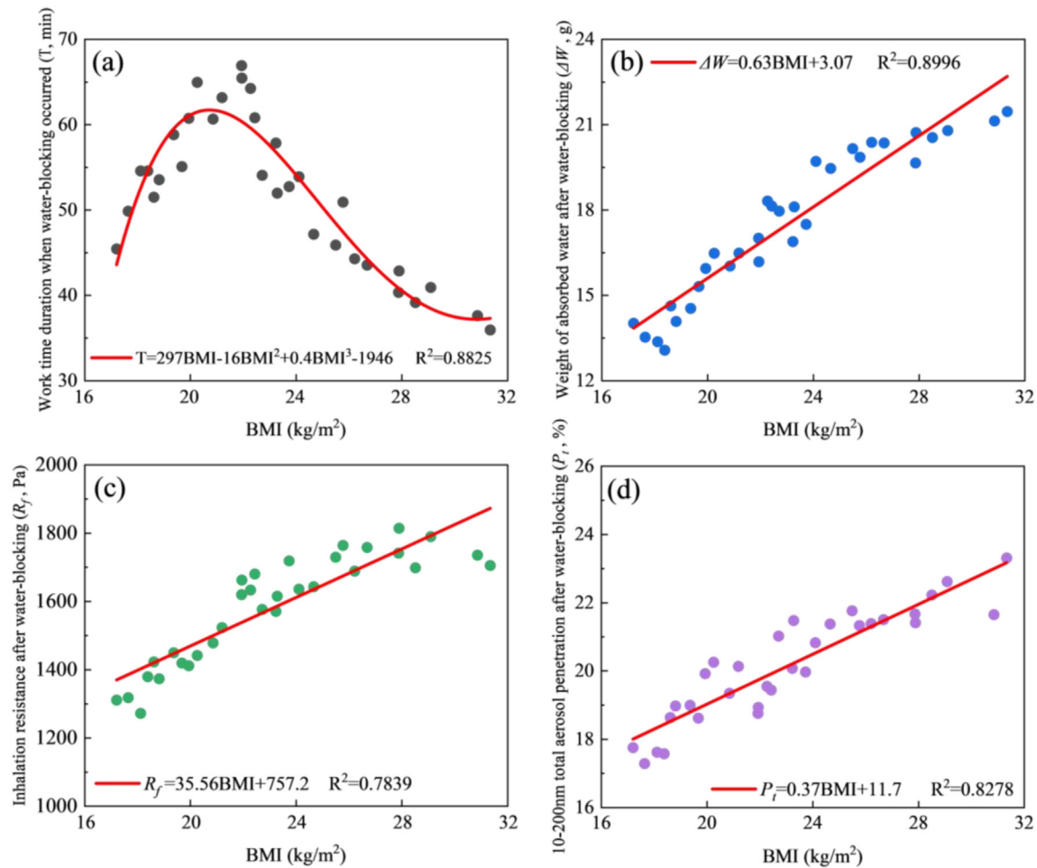
Fig. 6. Relationship between work time duration ( T ), weight of absorbed water ( \Delta W ), inhalation resistance ( R_f ), 10–200 nm total aerosol penetration ( P_t ) and subjects' BMI when respirator water-blocking occurred.
